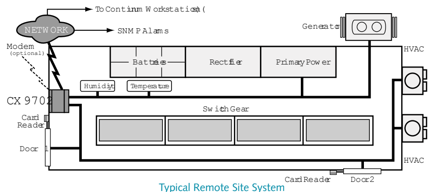
Typical Remote Site System
