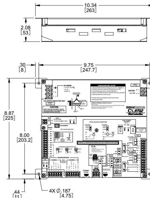
DIMENSIONAL DRAWINGS
